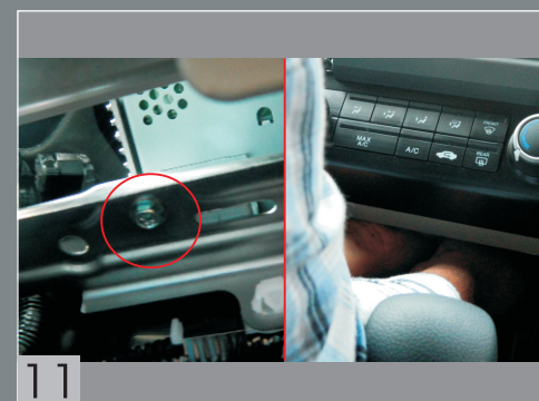
11 Take out the two fixed screws below original CD host.
