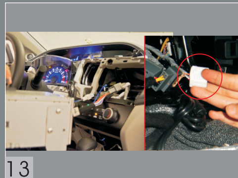
13 Connect the cables with car navigation, the white wire no need to connect.
