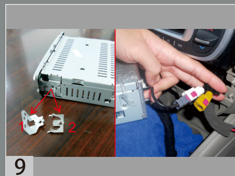
9 Fix the original side bracket on the unit, and connect the radio antenna (in the back of the DVD loader) to the original white connector.
