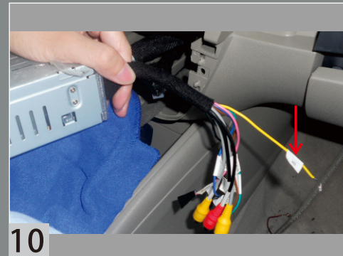
10 Connect the CCD+12V-OUT cable (shown on picture) to camera power cable.
