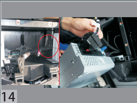
Connect the USB cable and the GPS antenna, then fish the USB cable to the glove box and put the antenna in right position.
