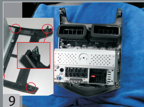
Assemble the air outlets and clips on the unit.
