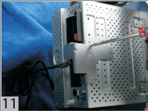
Fix the bracket C with screws.
